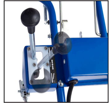
Quickly raise and lower edger for transport on and off the ice.
